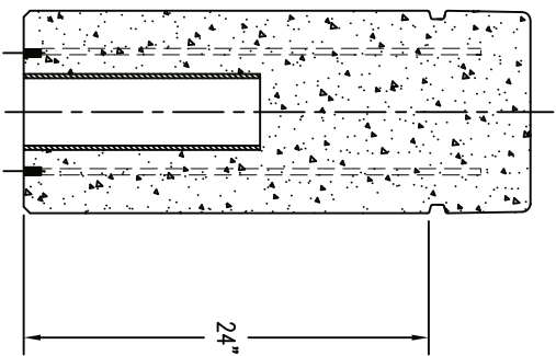
4 CROSS SECTION
