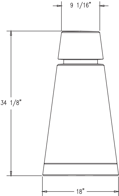
ELEVATION VIEW
