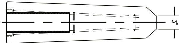
CROSS SECTION
