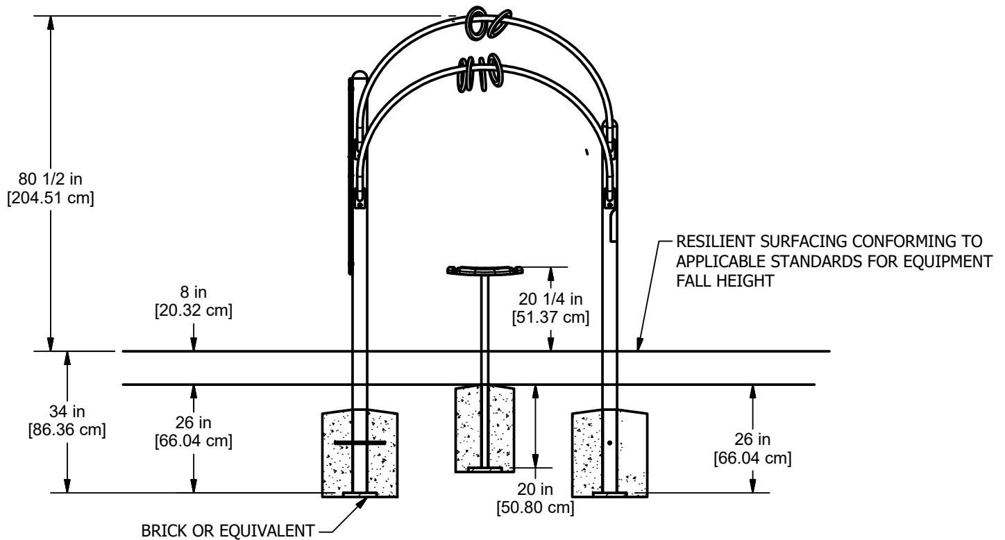
ELEVATION VIEW
