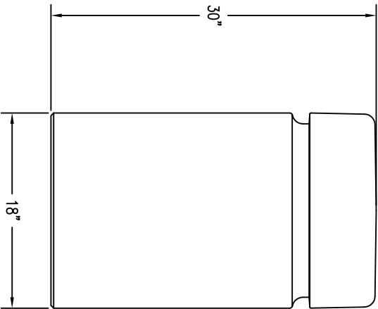
2 ELEVATION VIEW
