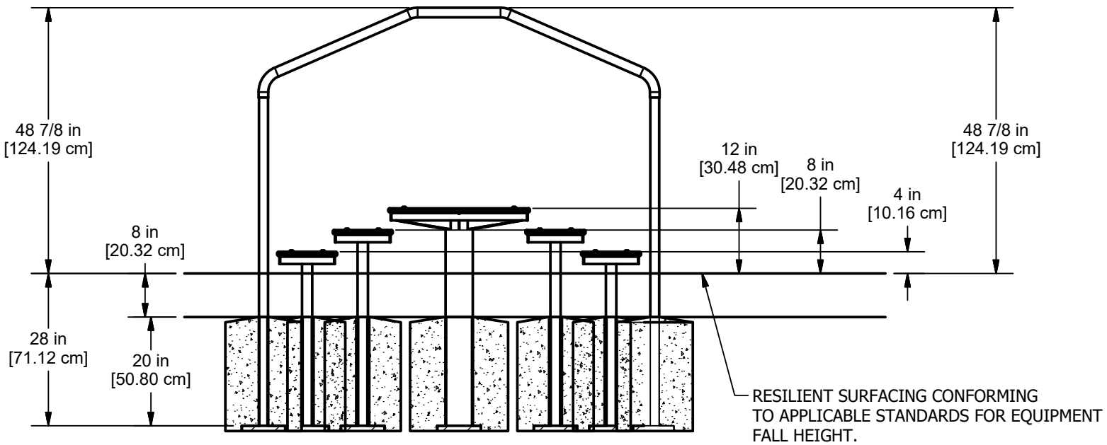
ELEVATION VIEW
